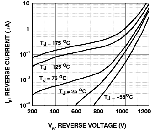
Figure 2. Reverse Characteristics
